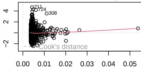
Residuals vs Leverage
